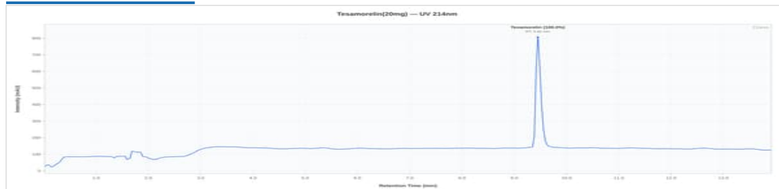
TSM 20mg - TES020-02: UV Chromatogram
