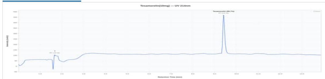
TSM 10mg - TES0123-02: UV Chromatogram
