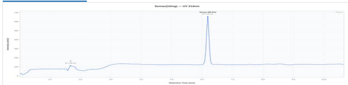
Semax 10mg - SEM123-03: UV Chromatogram
