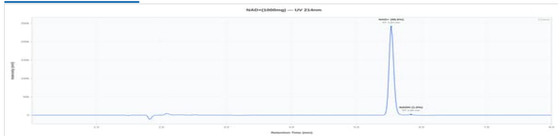
NAD+ 1000mg - NAD1000-02: UV Chromatogram
