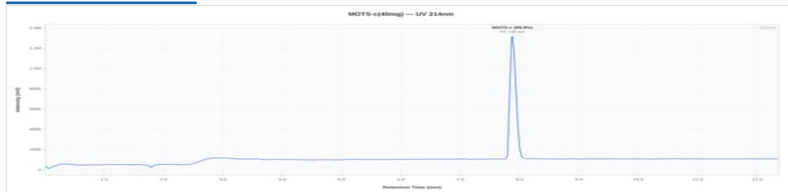
MOTS-C 40mg - MTC40-02: UV Chromatogram
