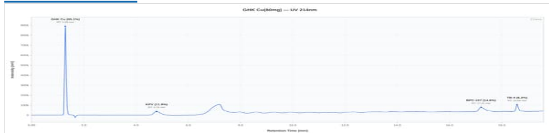
Klow 80mg - KLOW123-02: UV Chromatogram
