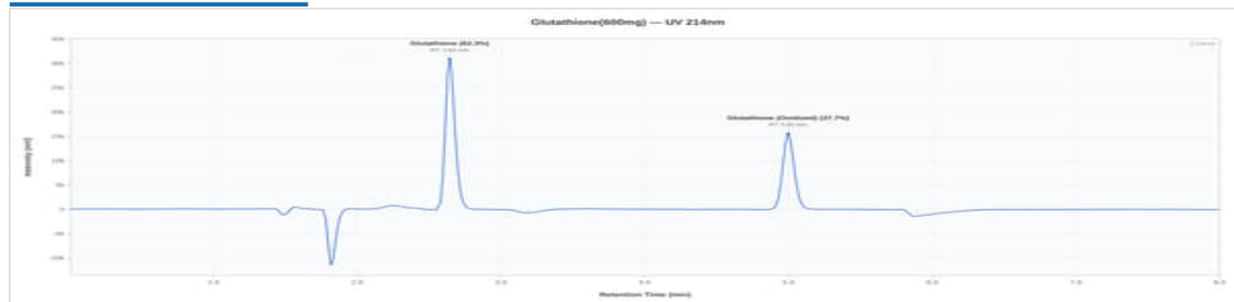
Glutathione 600mg - GLU600-02: UV Chromatogram
