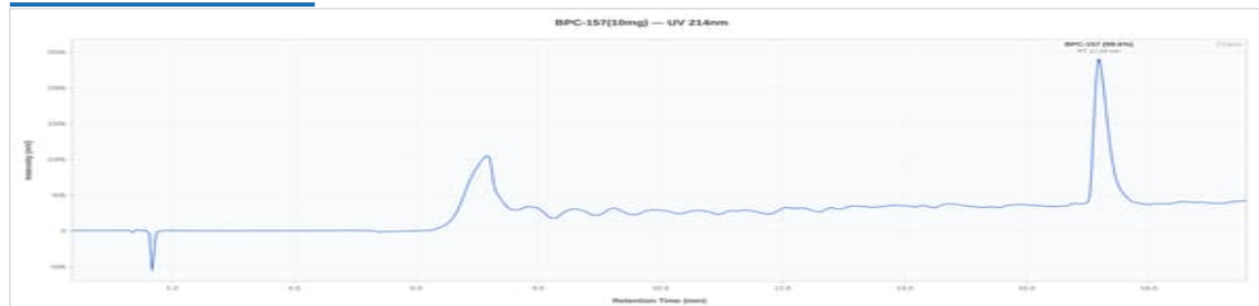
BPC-157 10mg - BPC157-03: UV Chromatogram
