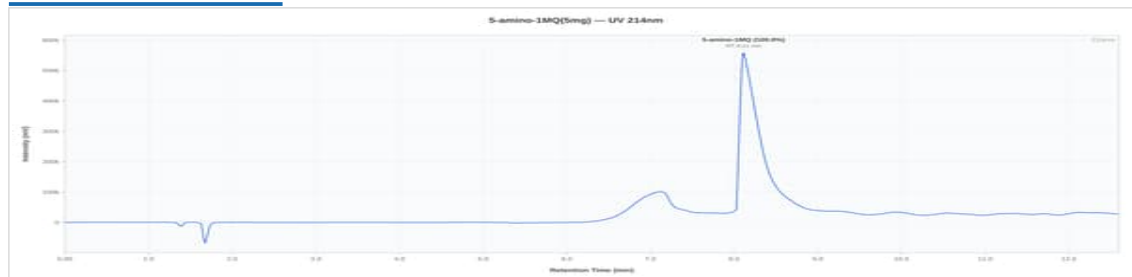
5-Amino-1MQ 5mg - 5Amino-02: UV Chromatogram
